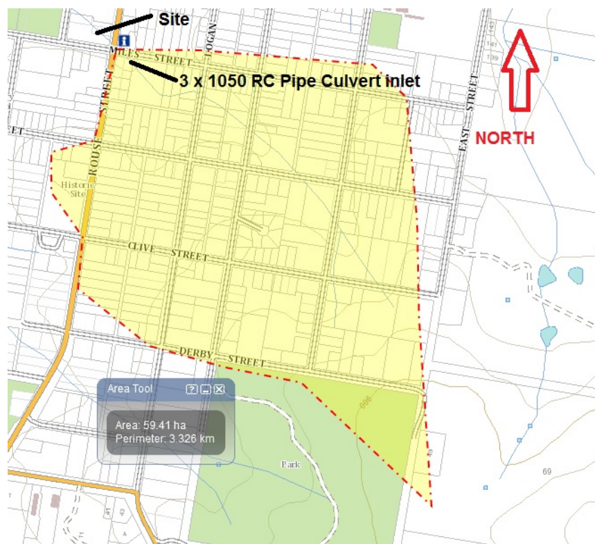
Image 1 Catchment area for existing culvert system
