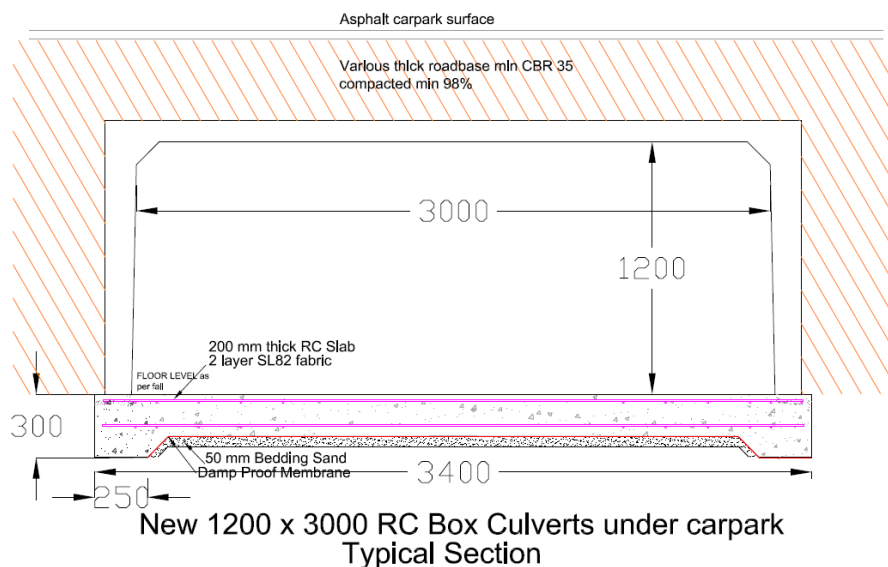
Image 4 Concept cross section of Proposed Reinforced Concrete Box culverts under Carpark
