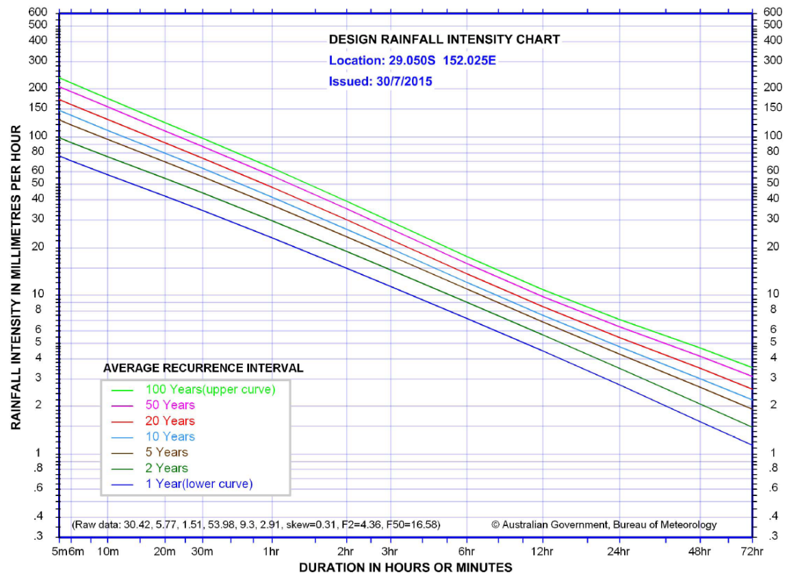
Image A1 IFD Chart Tenterfield
