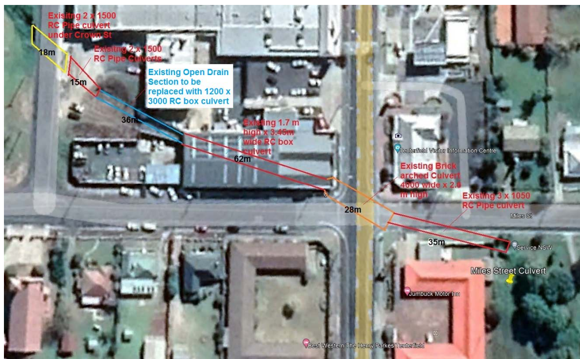
Image 2 Site Layout.
